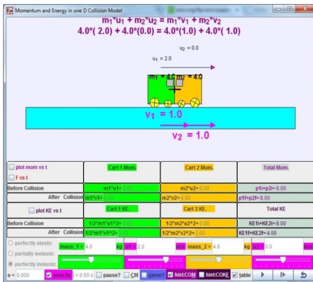
Figure 4. Collision cart
