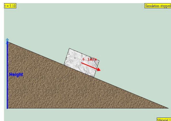
Customized simulation
