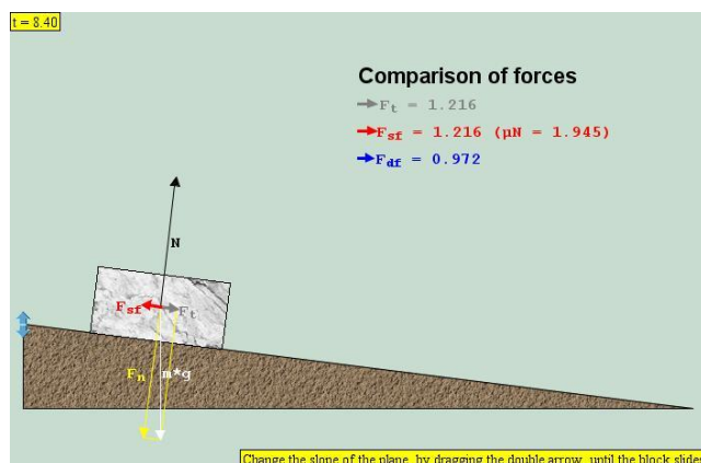
Original simulation
