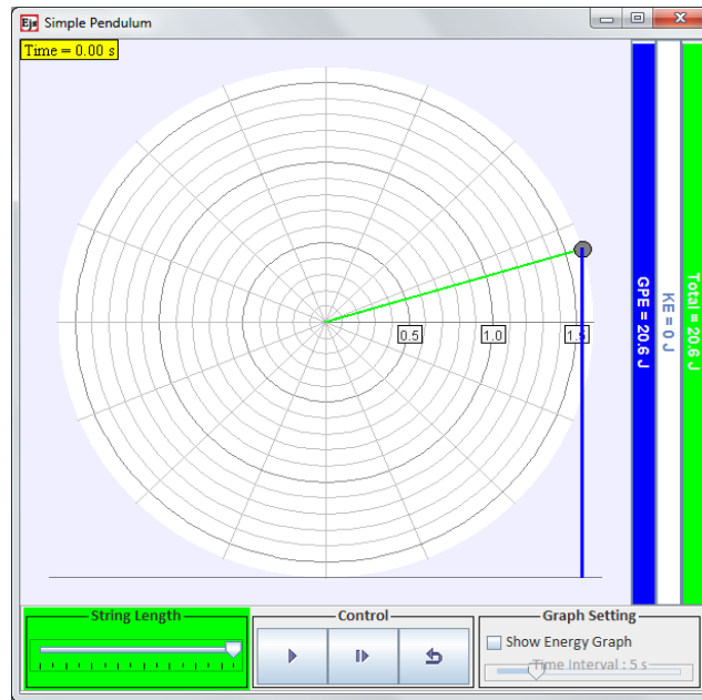
Figure 2. Pendulum simulation
