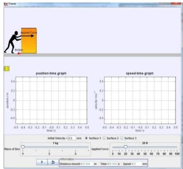
Figure 5. Friction simulation
