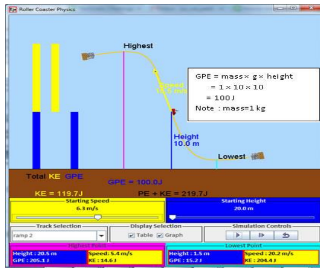
Figure 7. Energy law in roller coaster simulation
